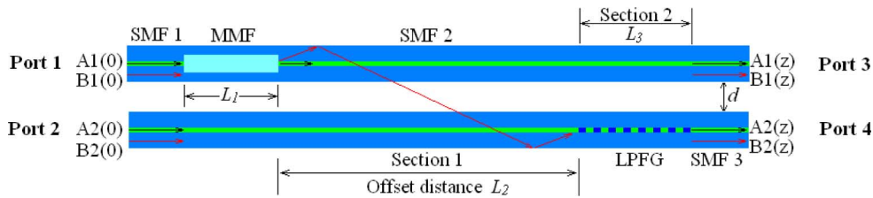
Fig. 1. Coupling configuration between an SMS fiber structure and an LPFG.
