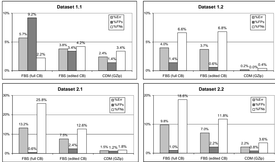
Fig. 1. Comparison between feature-based similarity (FBS) and compression-based similarity, using 10-fold cross validation on each dataset.
