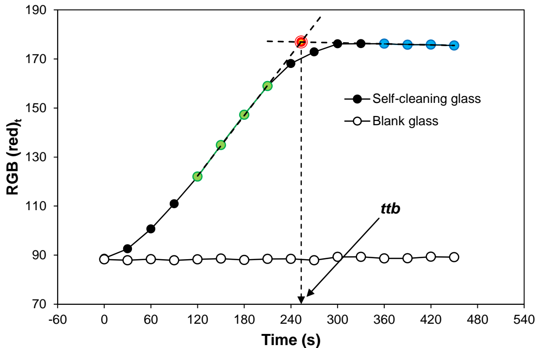
Fig. 2. – (a) A series of images recorded at 30 second irradiation intervals for two glass samples, namely; self-cleaning glass (top) and, plain glass (bottom). (b) A plot of variation of the RGB (red) with irradiation time, extracted from the images shown in (a). \text{RGB (red)}_t is the value of the RGB
