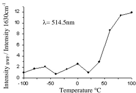
Fig 3. Intensity BWF/ Intensity 1630cm -1 as a function of temperature for HiPco composite at 514.5nm
