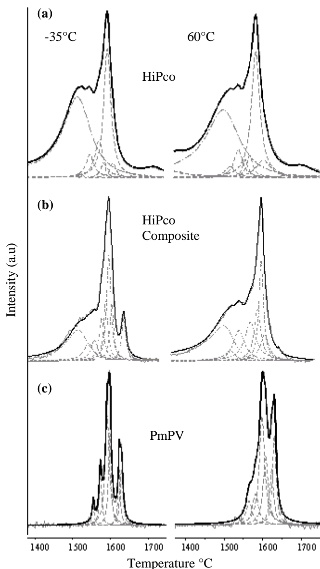
Fig 2. Temperature Dependent Raman spectra at 514.5nm at -35°C and 60°C of (a); Raw HiPco (b); 0.1% HiPco Composite and (c); PmPV
