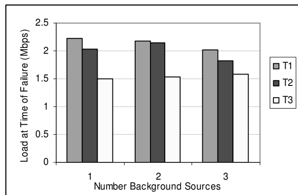
Figure 6. Mean failure times with packet size and number of contributing sources
