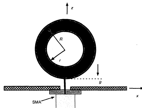
Fig. 1 Geometry of annular planar monopole antenna
