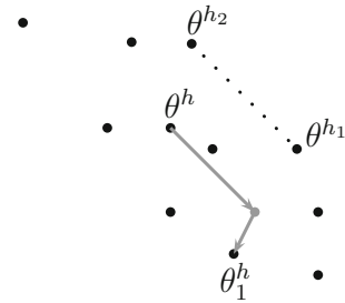
Fig. 1 The move of \theta^h is generated from the difference \theta^{h_1} - \theta^{h_2} plus a random term \epsilon
