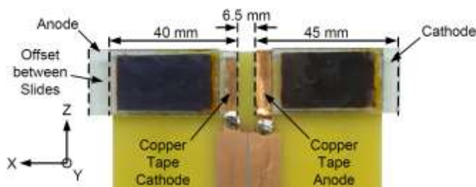
Fig. 1 – Rear of dye-Sensitised Solar Dipole Antenna
