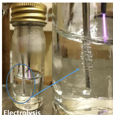
Figure 13. Oxygen bubbles around the anode rod during glow discharge
