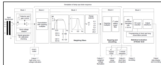
Figure 6: Block Diagram of Flickermeter from [2]
