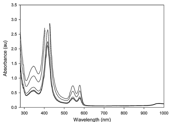
Fig. 3. Absorption spectra of whole blood from six donors evaluated from 280 to 1000 nm.
