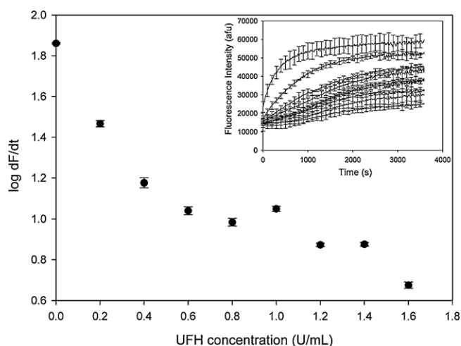
Fig. 1. Log/lin dose–response curve of UFH within the range of 0–1.6 U/mL in human pooled plasma. Inset: reaction progress curves of the ANSN-based fluorogenic anti-FXa assay (100 nM FXa and 25 \mu M ANSN fluorogenic substrate) using human pooled plasma spiked with UFH (0–1.6 U/mL) ( n = 3 ).
