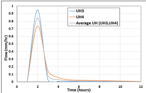
Figure 2. Comparison of three UHs at the River Slang Catchment.
