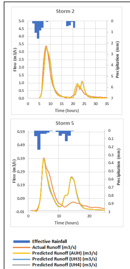
Figure 7. Predicted and actual flow hydrographs for the River Big Catchment.
