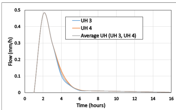
Figure 4. Comparison of three UHs at the River Big Catchment.
