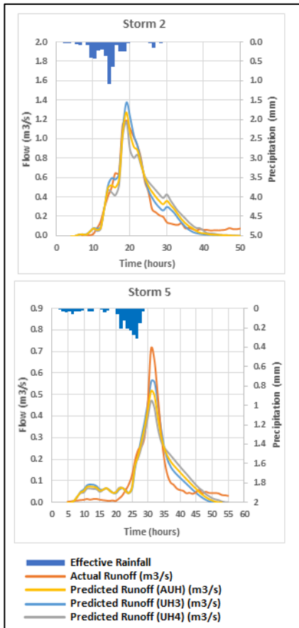
Figure 6. Predicted and actual flow hydrographs for the Lough Ennell Tributary River Catchment.
