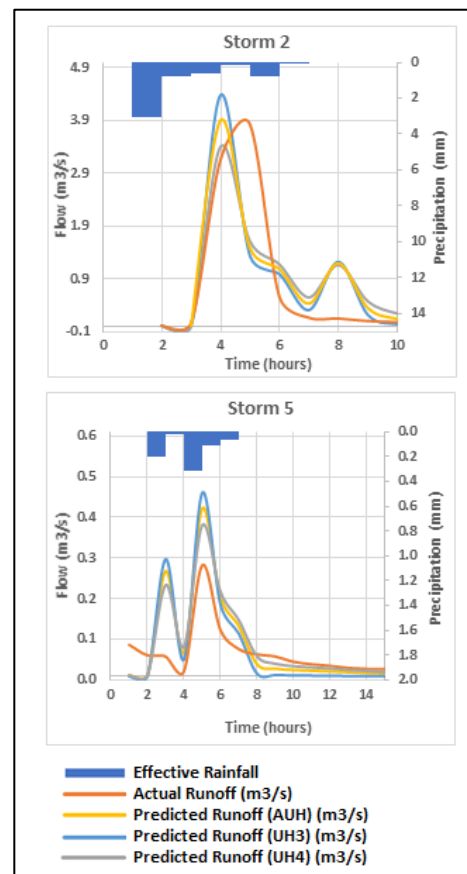
Figure 5. Predicted and actual flow hydrographs for the River Slang Catchment.
