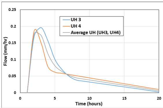
Figure 3. Comparison of three UHs at the Lough Ennell Tributary River Catchment.
