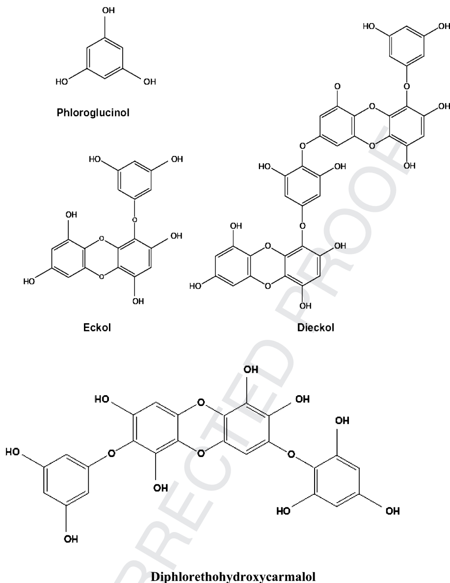
428 Fig. 3. Chemical structures of different types of phlorotannins (Heo et al. , 2009; 2010).
