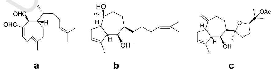
449 Fig. 4. Structure of Diterpenes isolated from brown algae (Manzo et al. , 2009) (a) Dictyodial; (b) Dictyol C; (c) Dictyol H.
