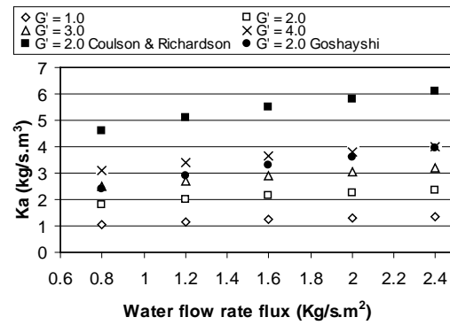
Figure 3 Volumetric total heat transfer coefficient for the test rig, as a function of water flow rate flux, for a series of air flow rate fluxes based on the experimental results. The comparison with the results of Goshayshi and Coulson & Richardson is also shown.
