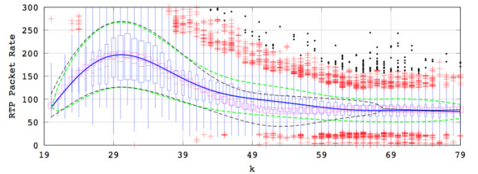
Figure 4. Predictions of the typical RTP packet rate and fluctuations in the RTP packet rate for a range of unseen values of the load 41 \leq k \leq 59 . The expected RTP packet loss for the missing data case, \bar{y}(k) , is indicated by pink squares. The expected fluctuations, \bar{\epsilon}_y(k) are indicated by black dashed lines.
