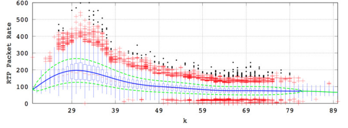
Figure 2. Boxplots and the 1st, 2nd, 3rd quartile of the underlying RTP packet rates as a function of the number of active users sessions k . The expected RTP packet rate \bar{y}(k) [blue] and \bar{\epsilon}_y(k) [green-dash] are also illustrated.
