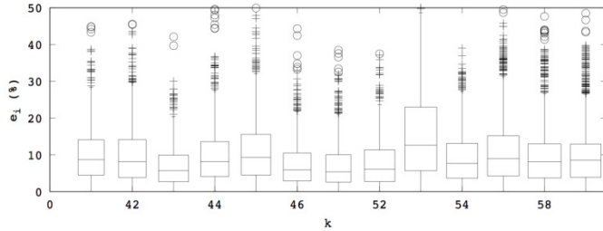
Figure 6. Boxplots (one for each value of k_{target} ) of the percentage absolute error for each predicted RTP packet rate.
