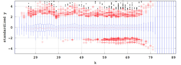
Figure 5. Effect of standardization on y_i . Irrespective of the load on the system, the samples are drawn from approximately the same distribution.
