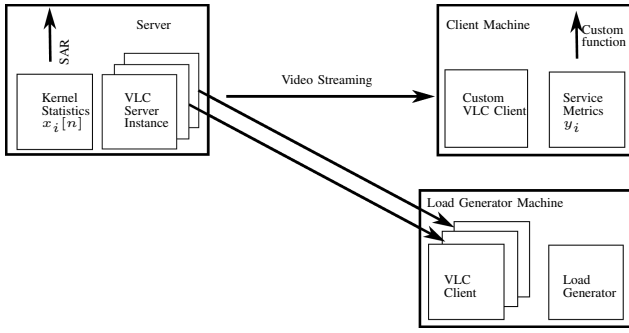
Figure 1. Prediction Scenario: A target client and multiple other clients (represented by the load-generating machine) share the video server's resources.
