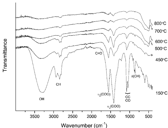
FIG. 6. FTIR spectra of Pb 0.5 Ba 0.5 TiO 3 powders with varied calcination temperatures ( T_c = 150, 450, 500, 600, 700, 800 °C).
