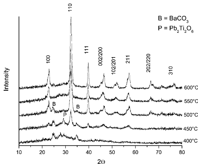
FIG. 4. X-ray diffraction patterns obtained from Pb 0.5 Ba 0.5 TiO 3 powder samples calcined at the temperatures indicated ( R_w = 8 , R_A = 4 ).
