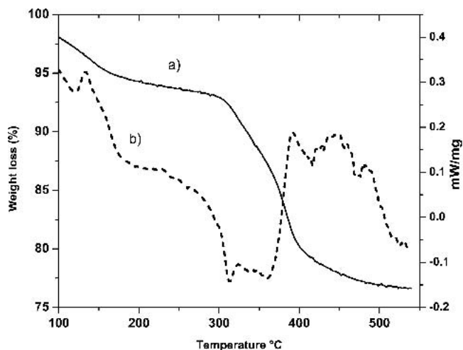
FIG. 5. (a) TGA and (b) DSC curves obtained from a Pb 0.5 Ba 0.5 TiO 3 powder sample prepared with R_w = 8 and R_A = 4 .
