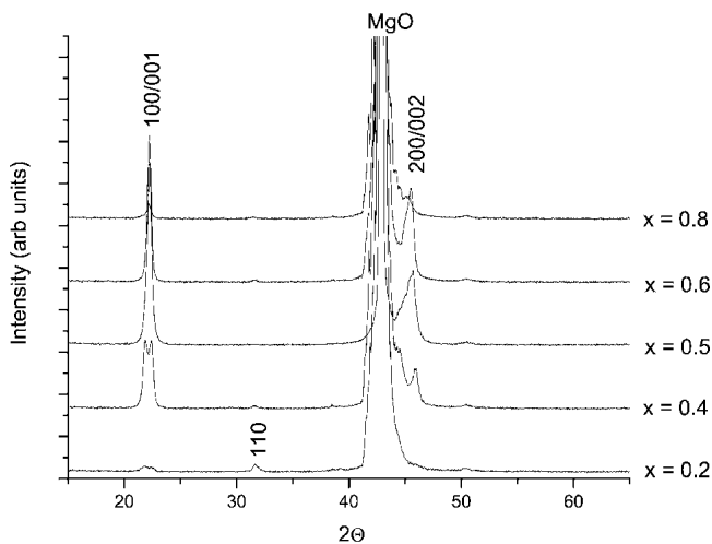
FIG. 9. X-ray diffraction patterns obtained from \text{Pb}_{1-x}\text{Ba}_x\text{TiO}_3 films with compositions as noted ( R_A = 4 , R_w = 8 , T_p = 450 °C, T_c = 600 °C, H_R = 5 °C/min).
