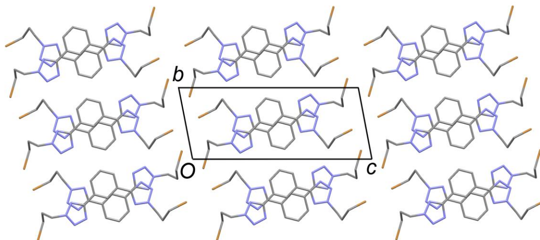
Figure 4. Projection of the crystal structure of 2 along the a axis, showing the layered structure with “Type II” Br \cdots Br contacts between layers. H atoms are omitted.
