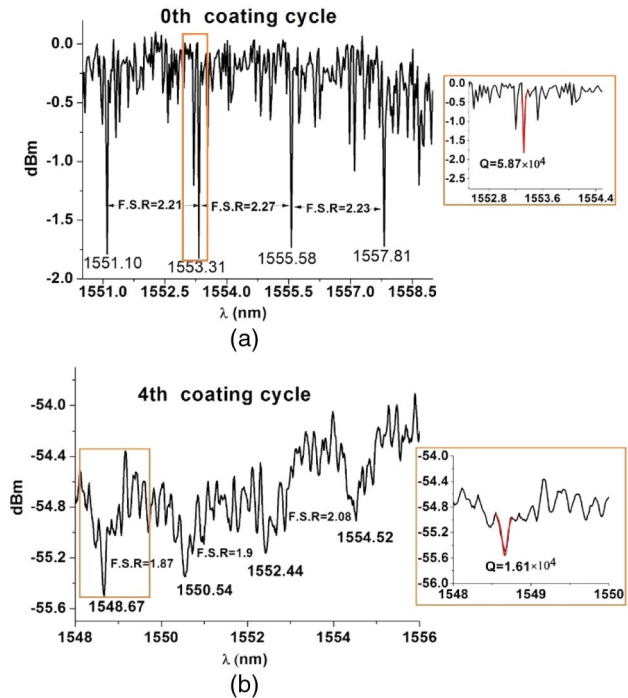
Fig. 5. Transmission spectra with the selected WGM resonances: (a) for uncoated silica microsphere with a 260 μm diameter and (b) for the same microsphere after application of four agarose coating layers. Insets illustrate fitting of the selected resonances and estimated Q -factors.
