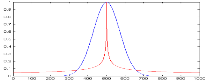
Figure 3. Comparison between a Gaussian distribution (blue) for \beta = 0.0001 and a Lévy distribution (red) for \gamma = 0.5 and p(0) = 1 .
