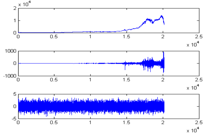
Figure 1. Financial time series for the Dow-Jones value (close-of-day) from 02-04-1928 to 12-12-2007 (top), the derivative of the same time series (centre) and a zero-mean Gaussian distributed random signal (bottom).
