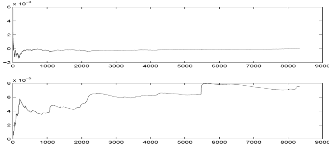
Figure 2. The first and second moments (top and bottom) of the Dow Jones Industrial Average plotted sequentially.
