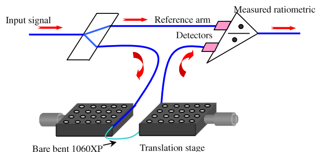
Figure 1. Experimental setup of the ratiometric measurement system which involves the proposed displacement sensor.
