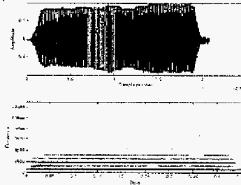
Figure 2: spectrogram of a tin whistle playing E 4
