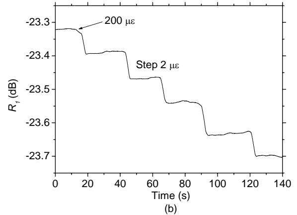
Fig. 5 Measured ratio R_1 variations vs. time with (a) step change 50 \mu\epsilon and (b) step change of 2 \mu\epsilon from 200 \mu\epsilon to 220 \mu\epsilon
