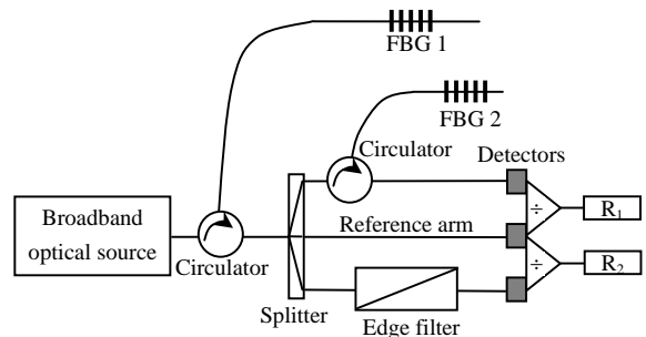
Fig. 6 Schematic diagram for simultaneous measurements of strain and temperature
