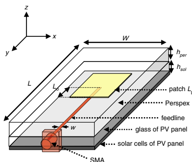
Fig. 1 Proposed antenna Dimensions W = 55 mm, L = 85 mm, L_p = 19 mm, L_o = 9.5 mm, w = 1.8 mm, h_{per} = 3 mm, h_{sol} = 2.3 mm
