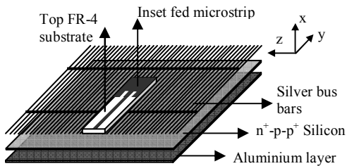
Fig. 1. Exploded layout of the inset-fed square patch solar antenna.
