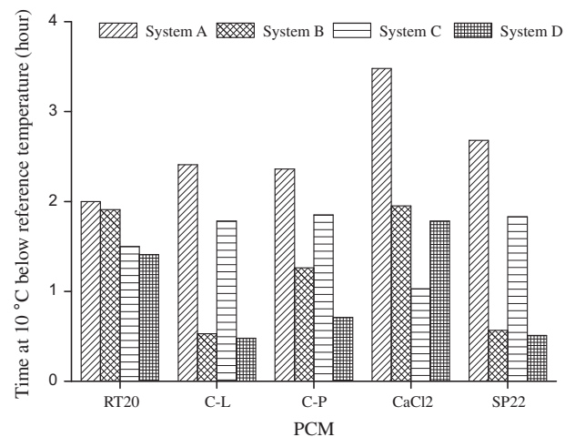
Fig. 8. Duration for which PCM maintained PV front surface temperature 10 °C below the reference temperature in systems A, B, C and D at an insolation of 750 W/m 2 and ambient temperature of 20 ± 1 °C.
