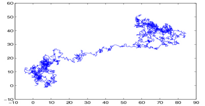
Fig. 7. Non-stationary random phase walk in the plane.
