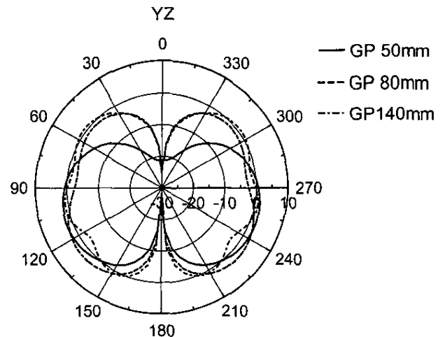
Figure 5c. The radiation patterns for the yz plane for ground-plane sizes of 50 \times 50 mm, 80 \times 80 mm, and 140 \times 140 mm.
