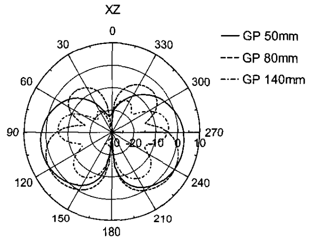
Figure 5b. The radiation patterns for the xz plane for ground-plane sizes of 50 \times 50 mm, 80 \times 80 mm, and 140 \times 140 mm.
