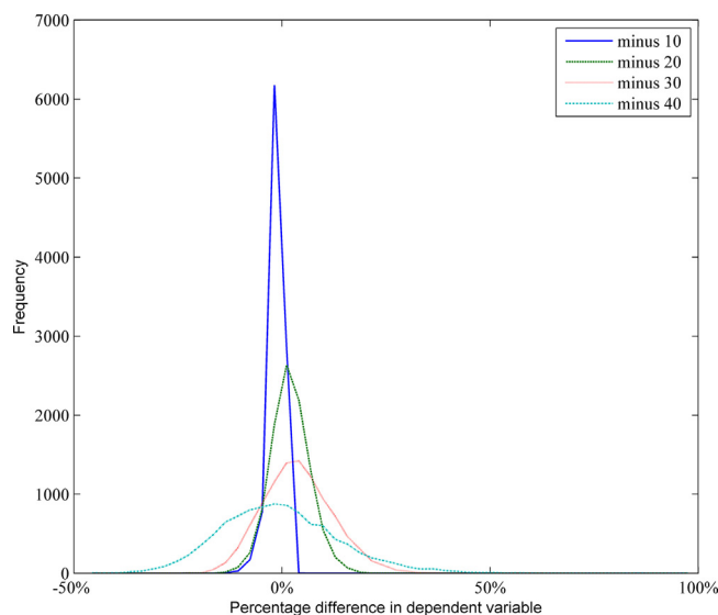
Fig. 2. Distribution of percentage variation between Zero Model and the four reduced versions of the ARM for the dependent variable (Primary energy per m 2 annum).
