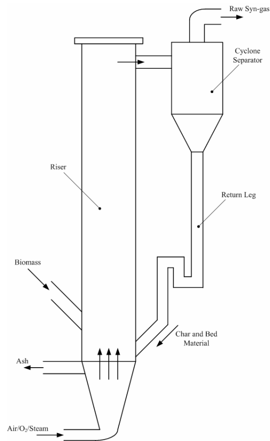
Fig. 1. Schematic diagram of a CFB biomass gasifier.
