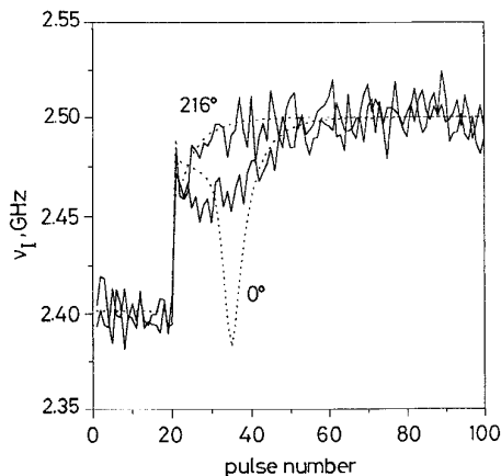
Fig. 5 Development of v_1 of SPLD during synchronisation to applied electrical signal of v_{APP} = 2.5\text{GHz} ..... No spontaneous emission noise, \Delta\Phi_{DI} = 0^\circ and 216^\circ — Average of 50 synchronisation runs, noise included
